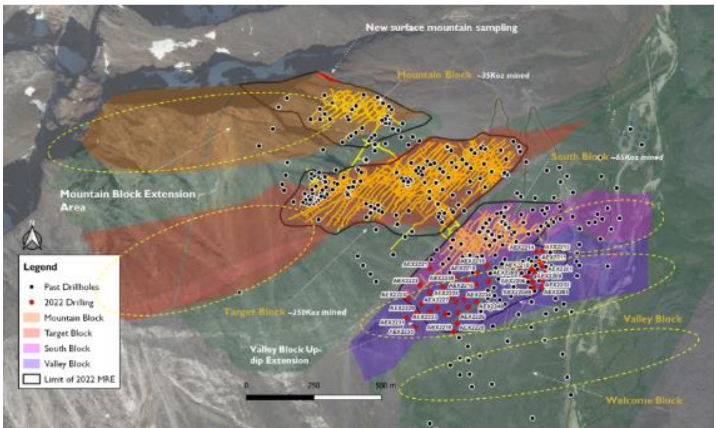
Figure 1. Nalunaq project map with 2022 drillhole locations
